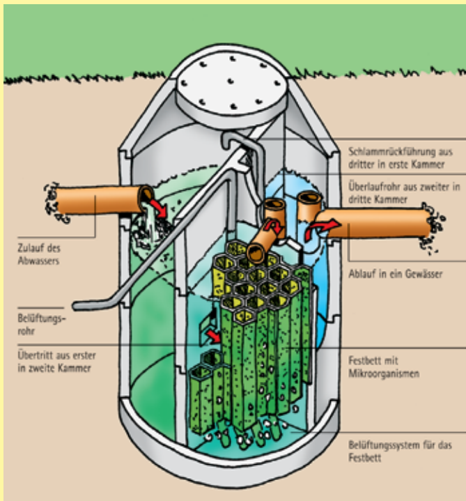
Abbildung 11: Festbetтанlage [13]
